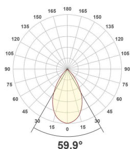
ES54284125_PD-28W-4000K
