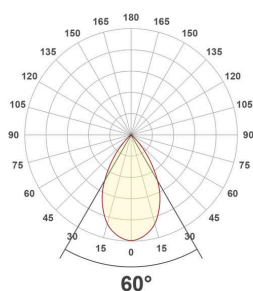
ES54284125_PD-28W-3000K
