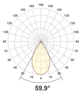
ES54284125_PD-24W-3000K
