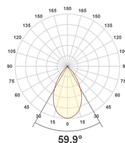
ES54284125_PD-28W-5700K
