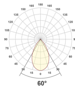
ES54284125_PD-24W-4000K
