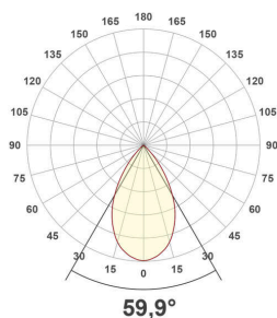
ES54284125_PD-18W-5700K
