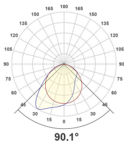
APS1500125AS_PD-32W-4000K
