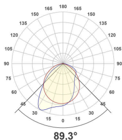
APS1500125AS_PD-37W-3000K
