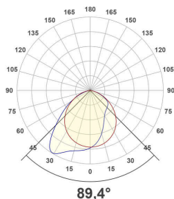
APS1500125AS_PD-32W-3000K
